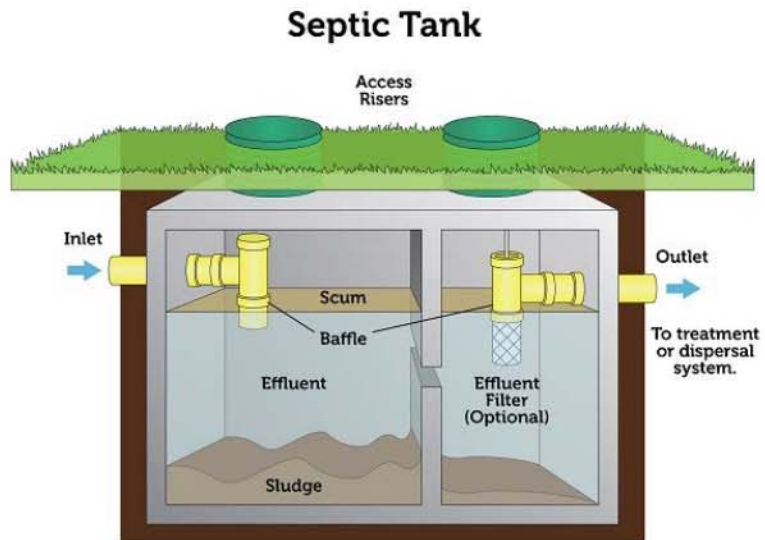
Figure 2: Septic tank.
