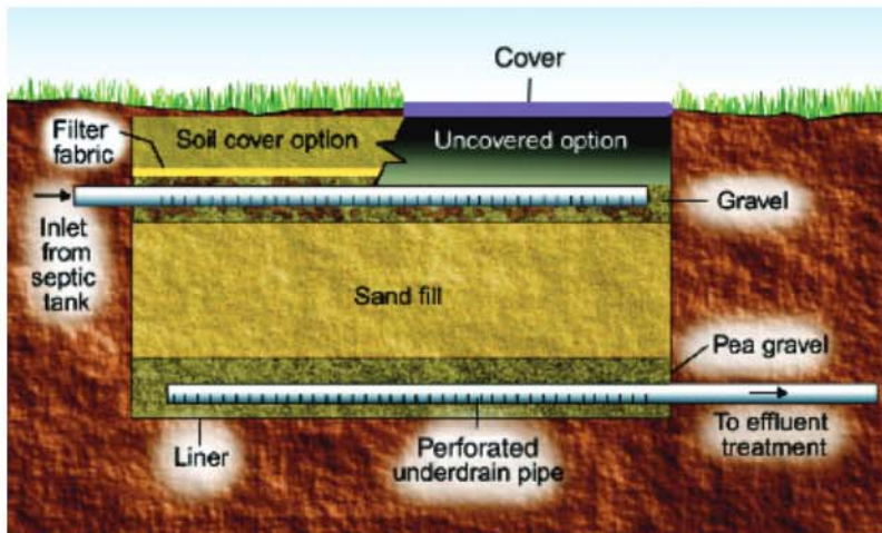
Figure 6: Sand filter.
